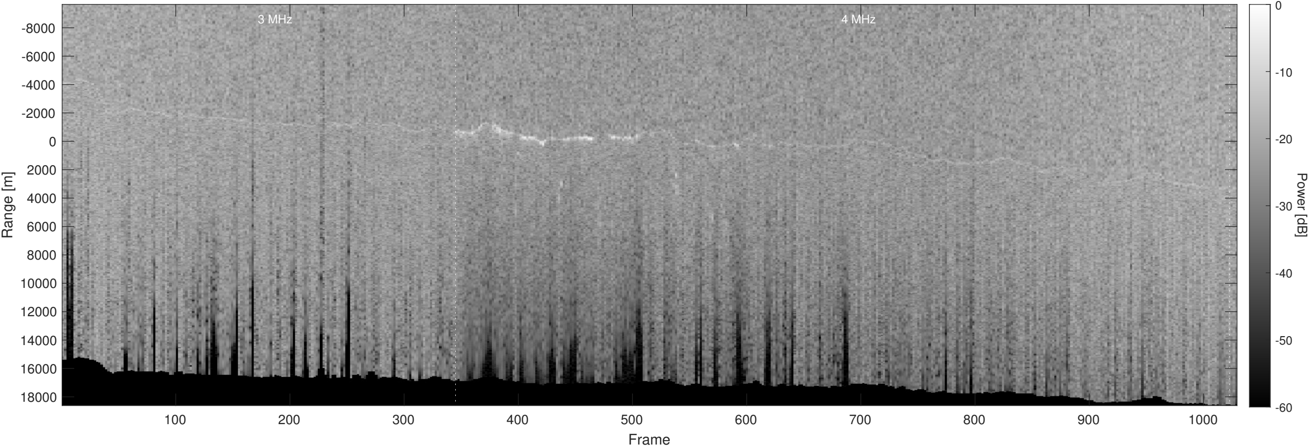
Orbit 12613, Optimized, No Window, Depth-Corrected, Channel 2
