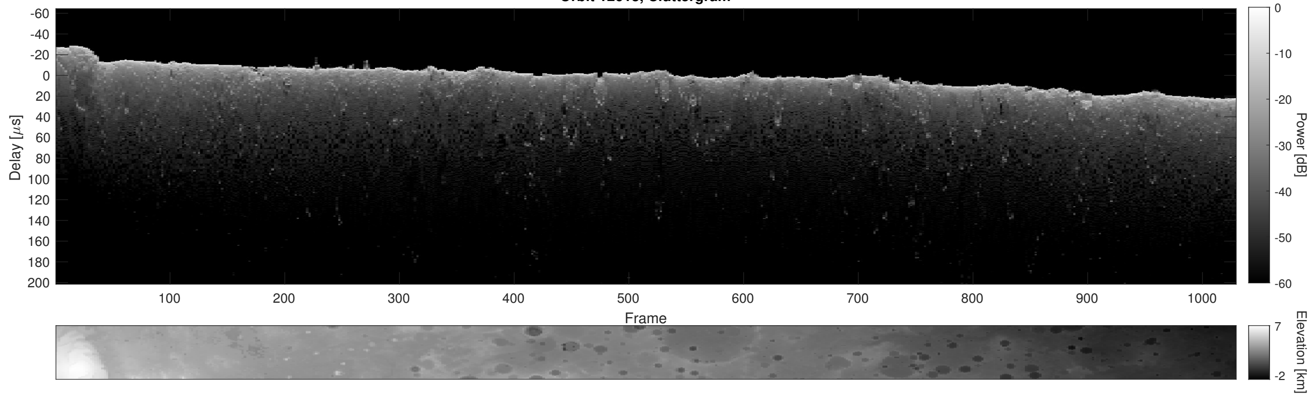
Orbit 12613, Cluttergram
