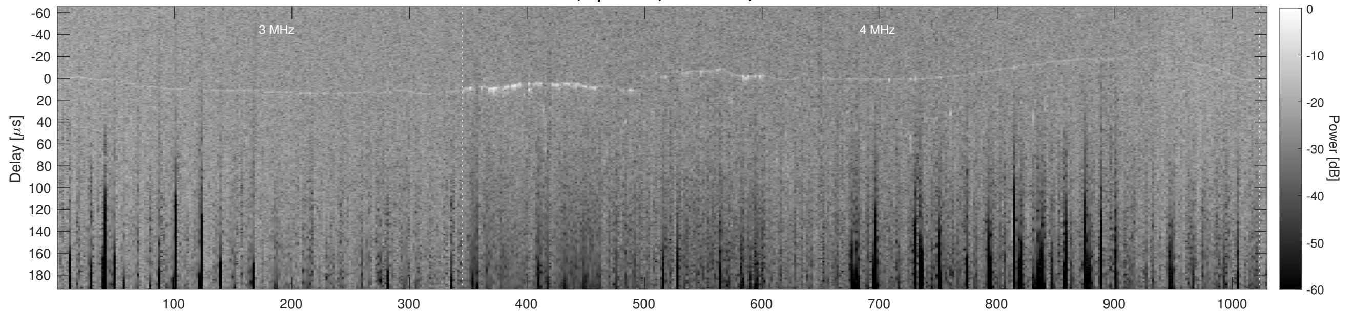
Orbit 12614, Cluttergram
