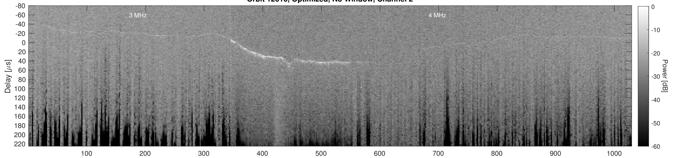
Orbit 12616, Cluttergram
