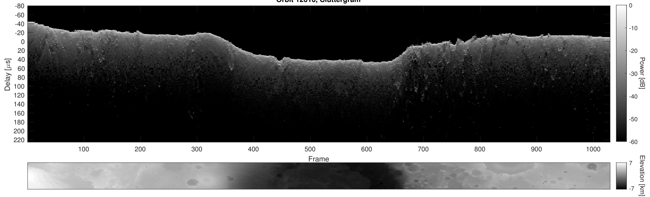
Orbit 12616, Cluttergram
