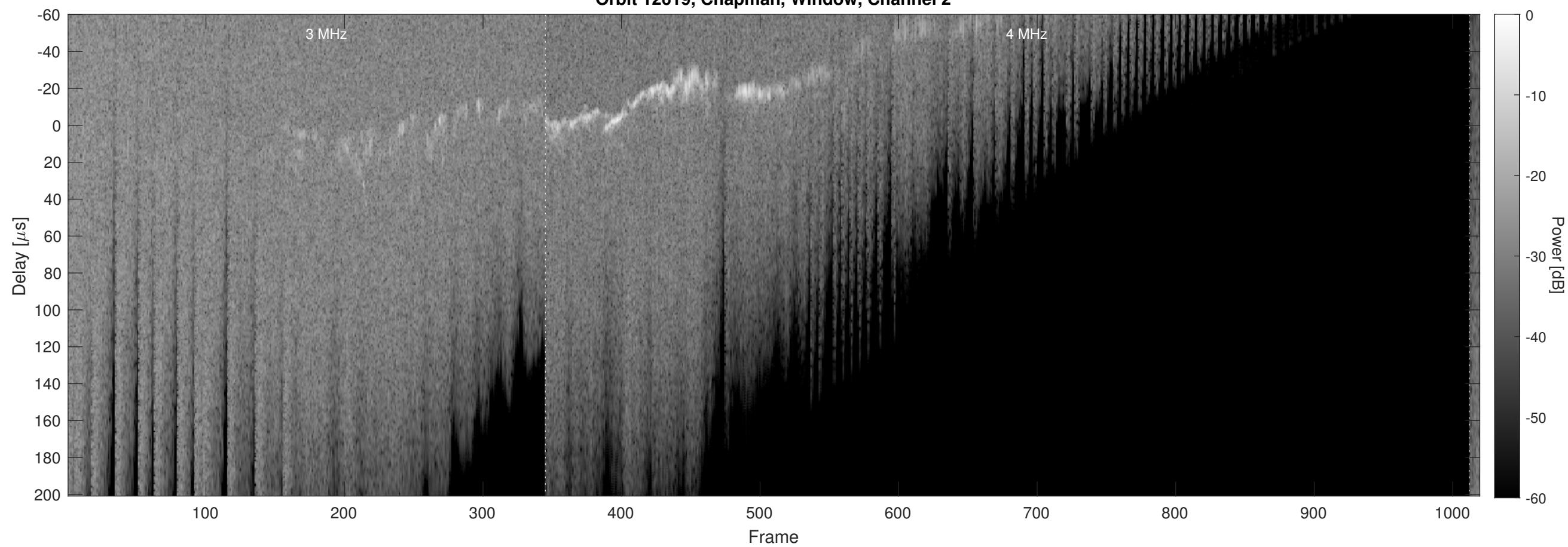
Orbit 12619, Chapman, Window, Channel 2
