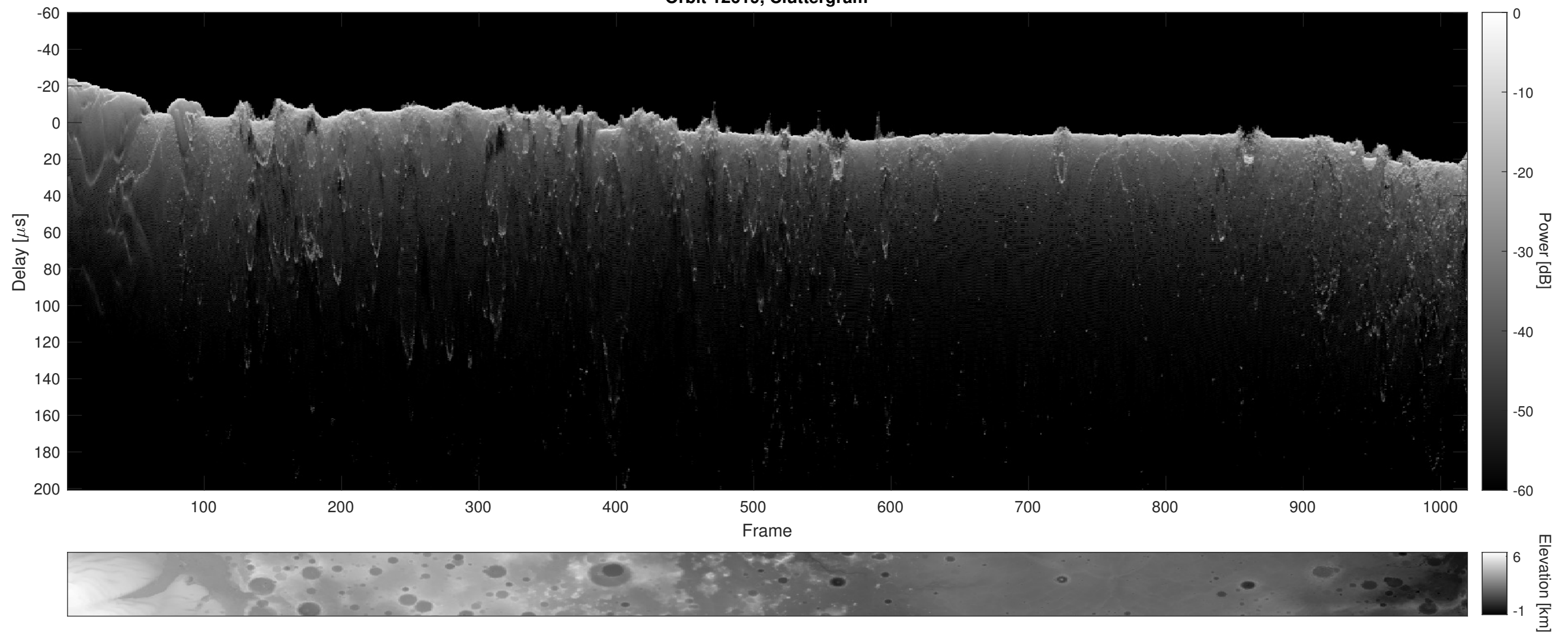
Orbit 12619, Cluttergram
