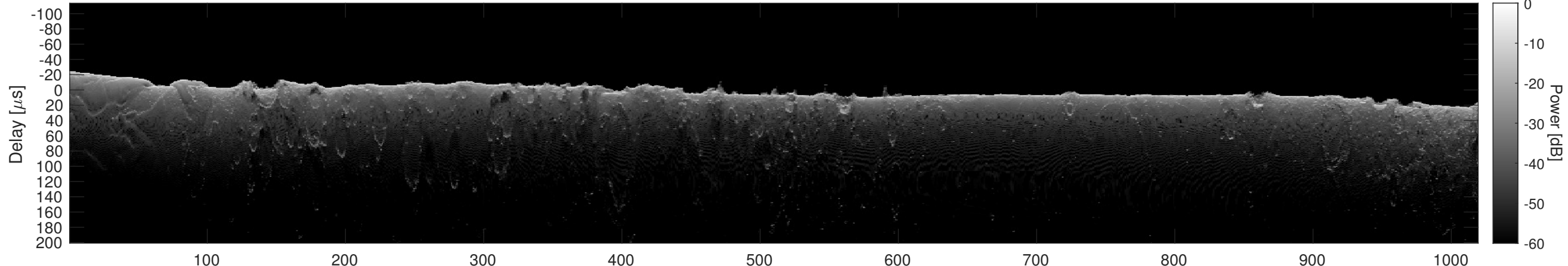
Orbit 12619, Cluttergram
