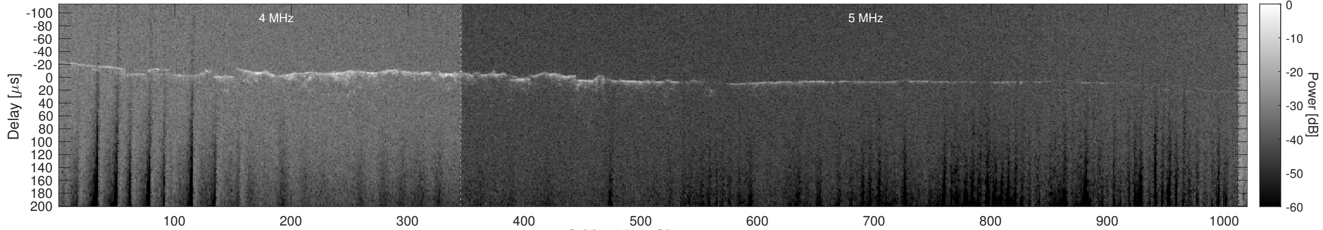
Orbit 12619, Cluttergram
