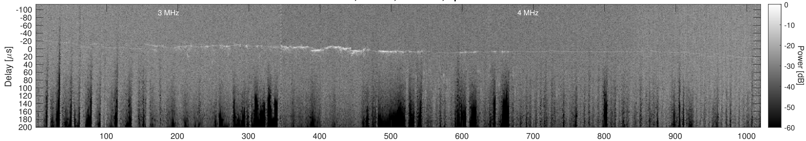
Orbit 12619, Cluttergram
