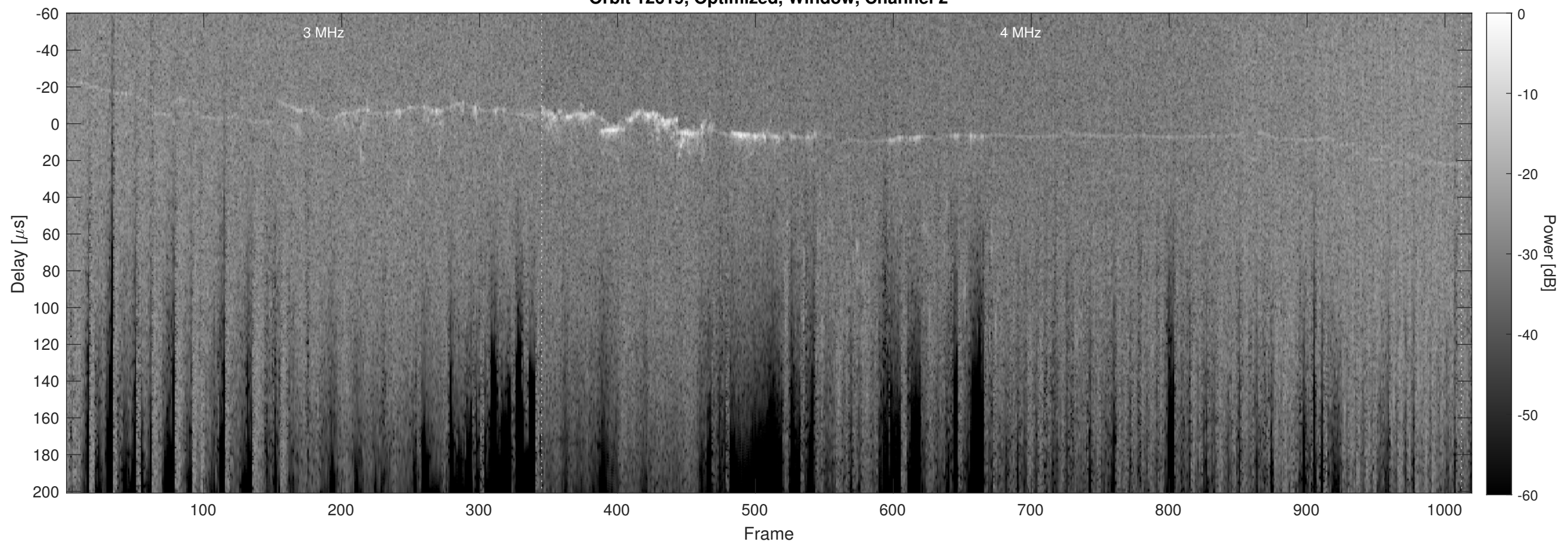
Orbit 12619, Optimized, Window, Channel 2
