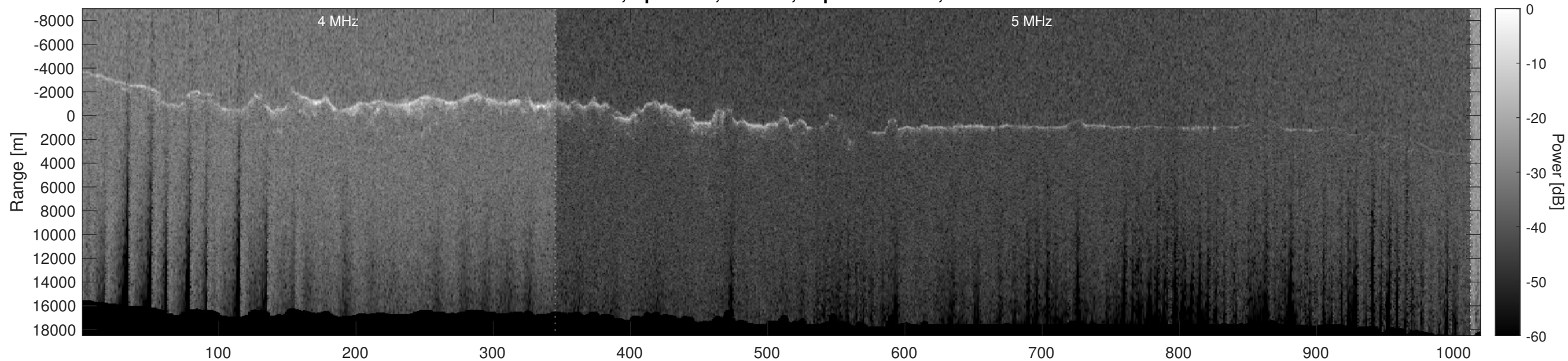
Orbit 12619, Optimized, Window, Depth-Corrected, Channel 2
