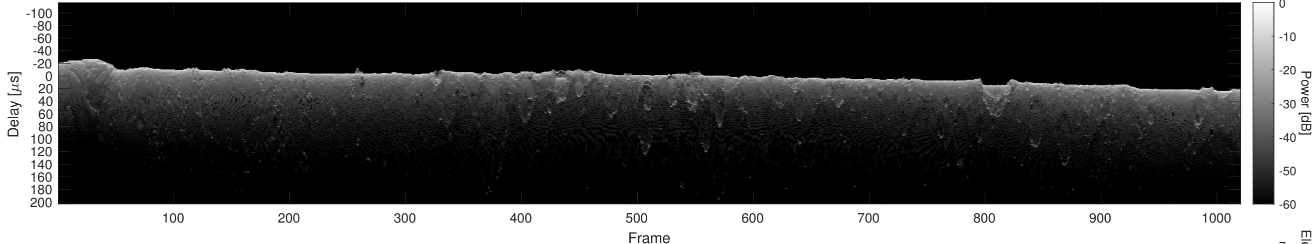
Orbit 12620, Cluttergram
