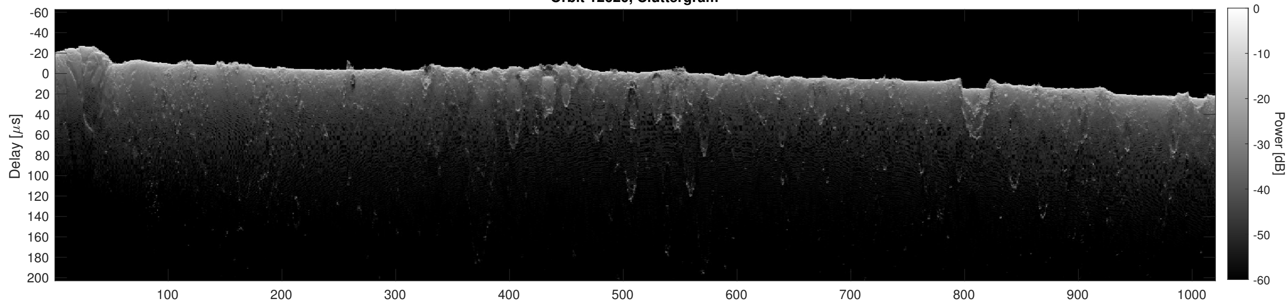
Orbit 12620, Cluttergram
