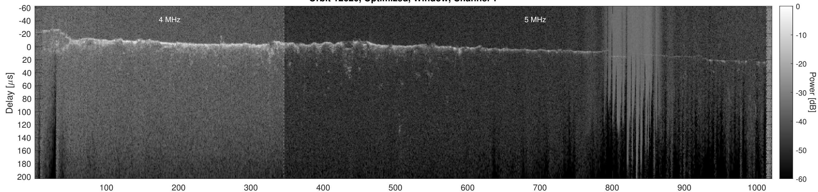
Orbit 12620, Optimized, Window, Channel 2
