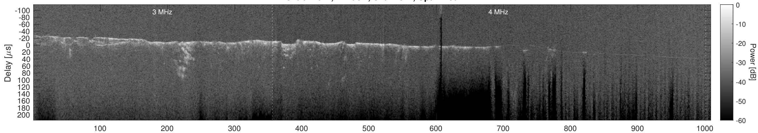
Orbit 12622, Cluttergram
