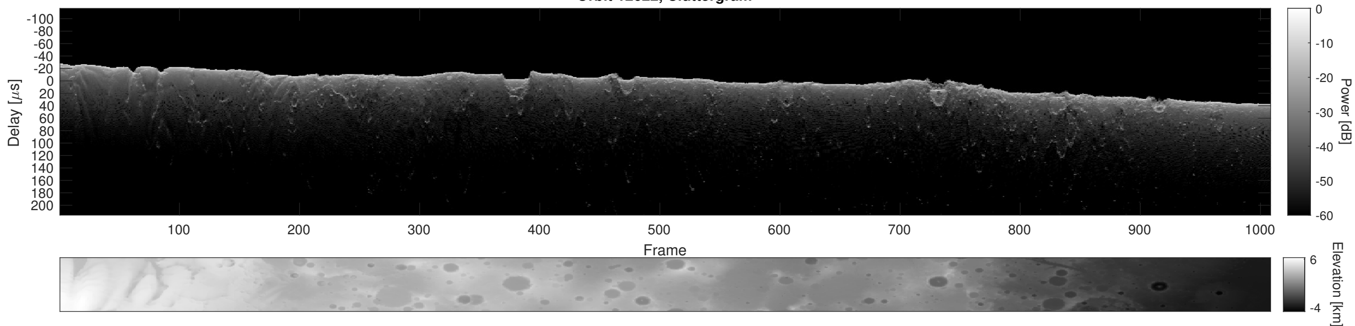
Orbit 12622, Cluttergram
