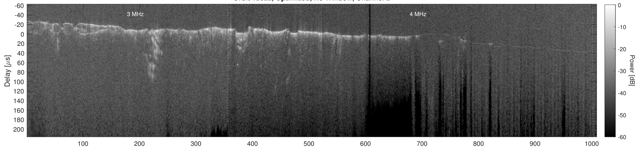
Orbit 12622, Cluttergram
