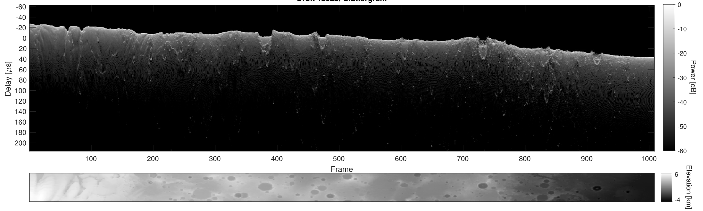
Orbit 12622, Cluttergram
