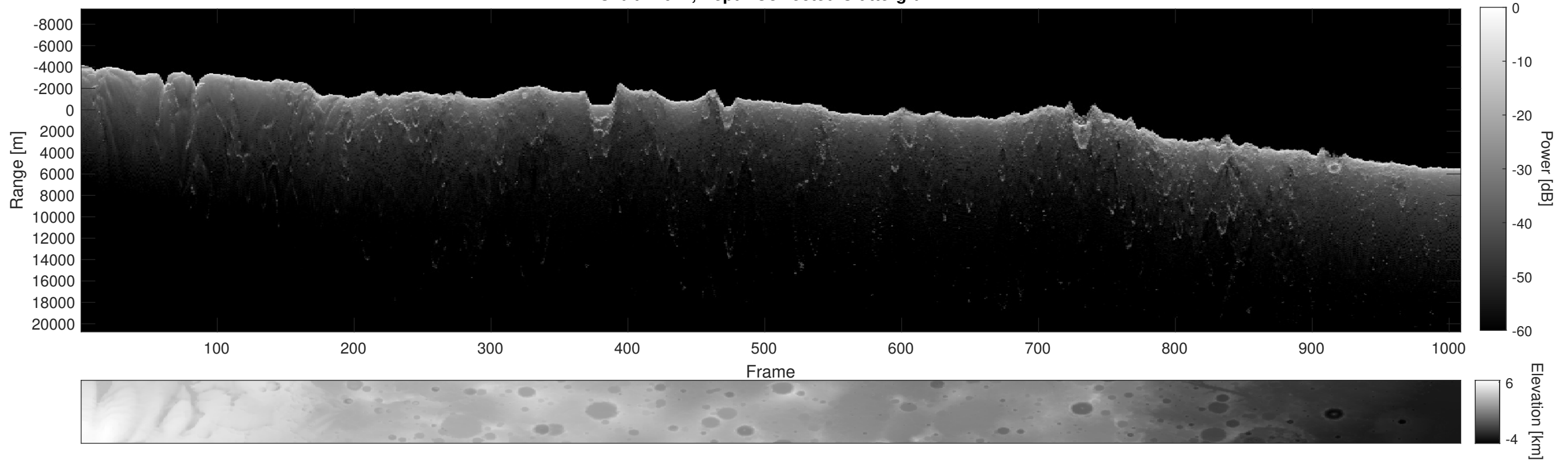
Orbit 12622, Depth-Corrected Cluttergram
