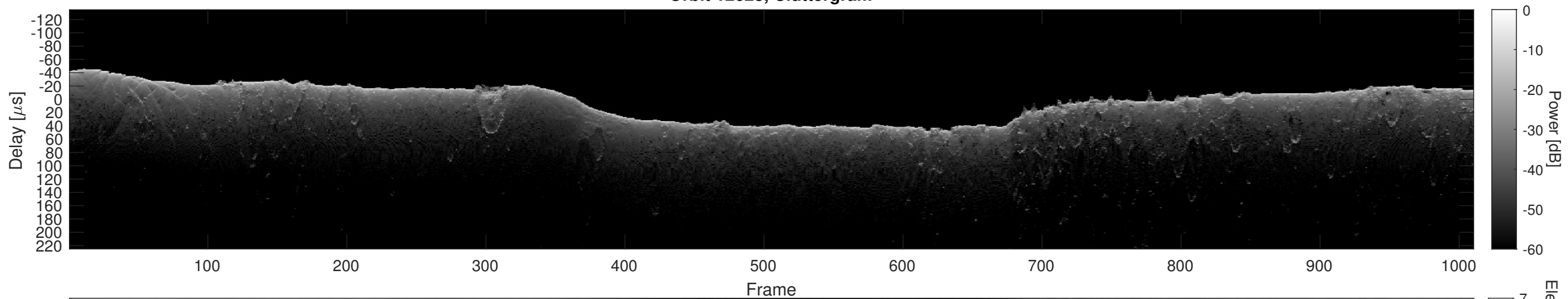
Orbit 12623, Cluttergram
