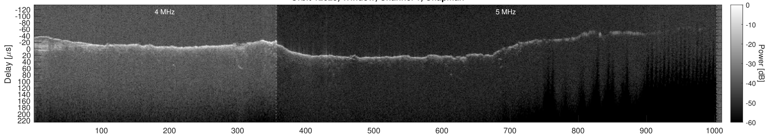
Orbit 12623, Window, Channel 1, Optimized
