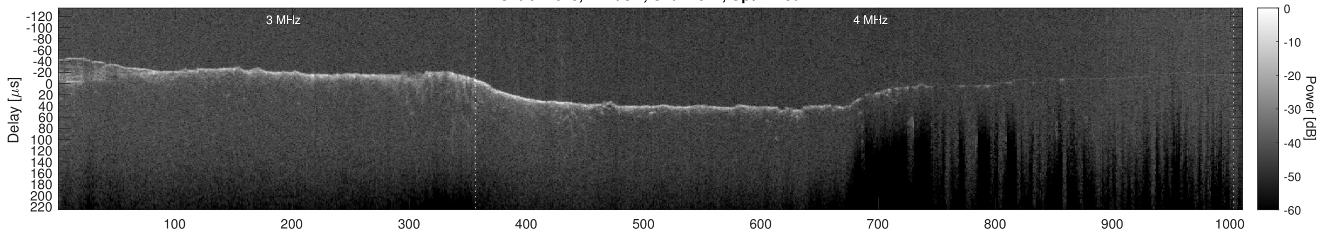
Orbit 12623, Cluttergram
