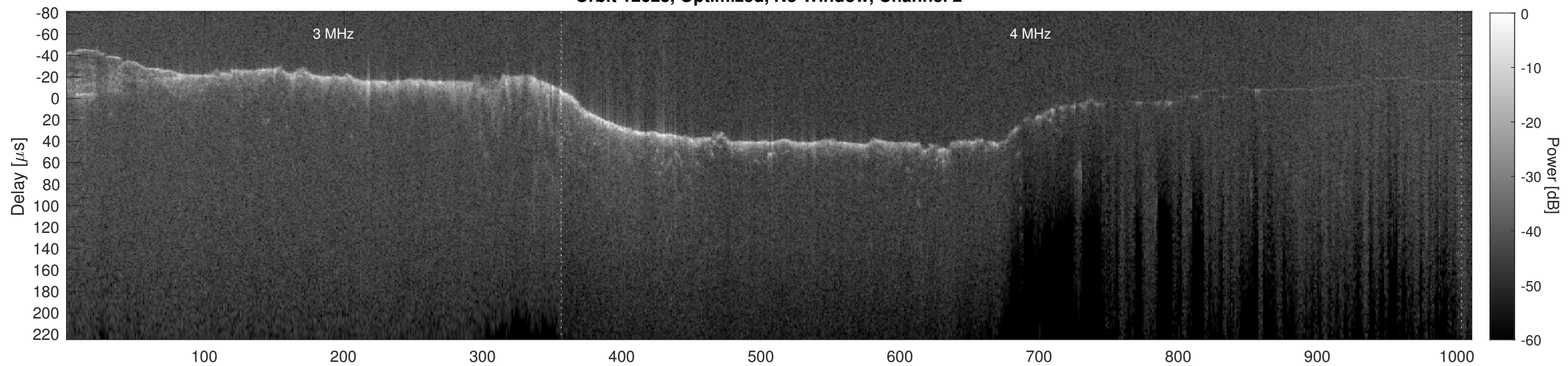
Orbit 12623, Cluttergram
