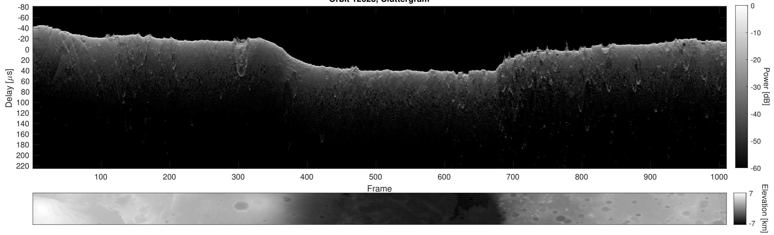
Orbit 12623, Cluttergram
