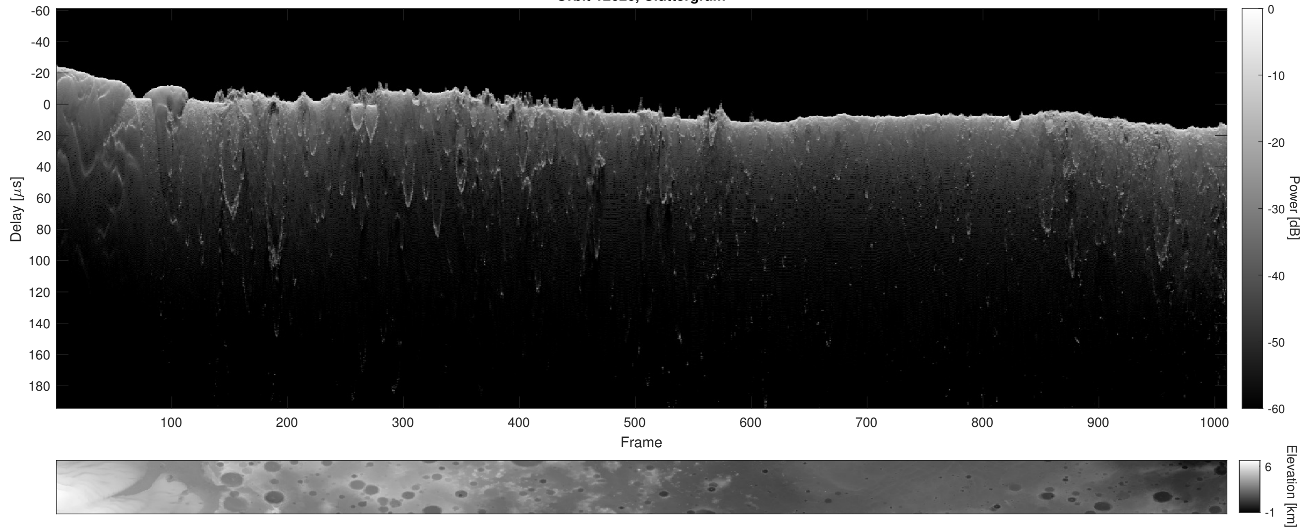
Orbit 12626, Cluttergram
