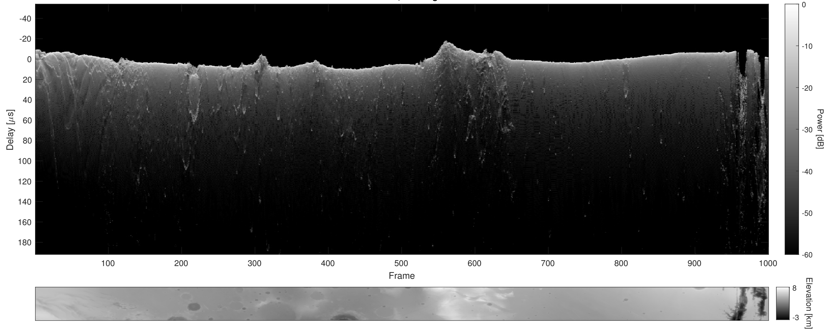
Orbit 12628, Cluttergram
