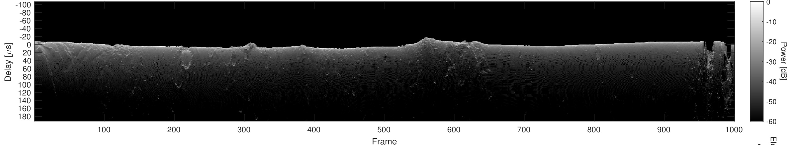
Orbit 12628, Cluttergram
