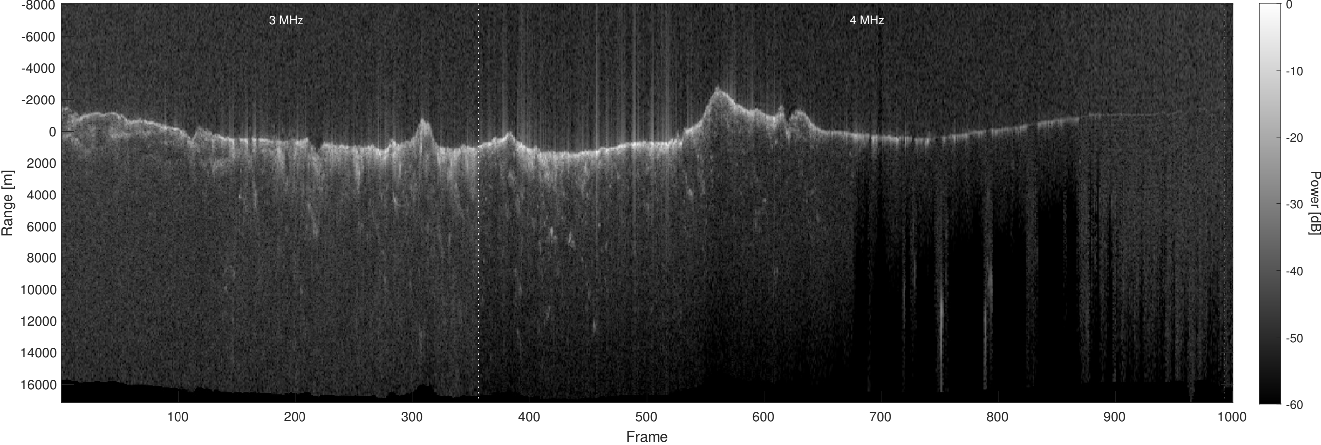
Orbit 12628, Optimized, No Window, Depth-Corrected, Channel 2
