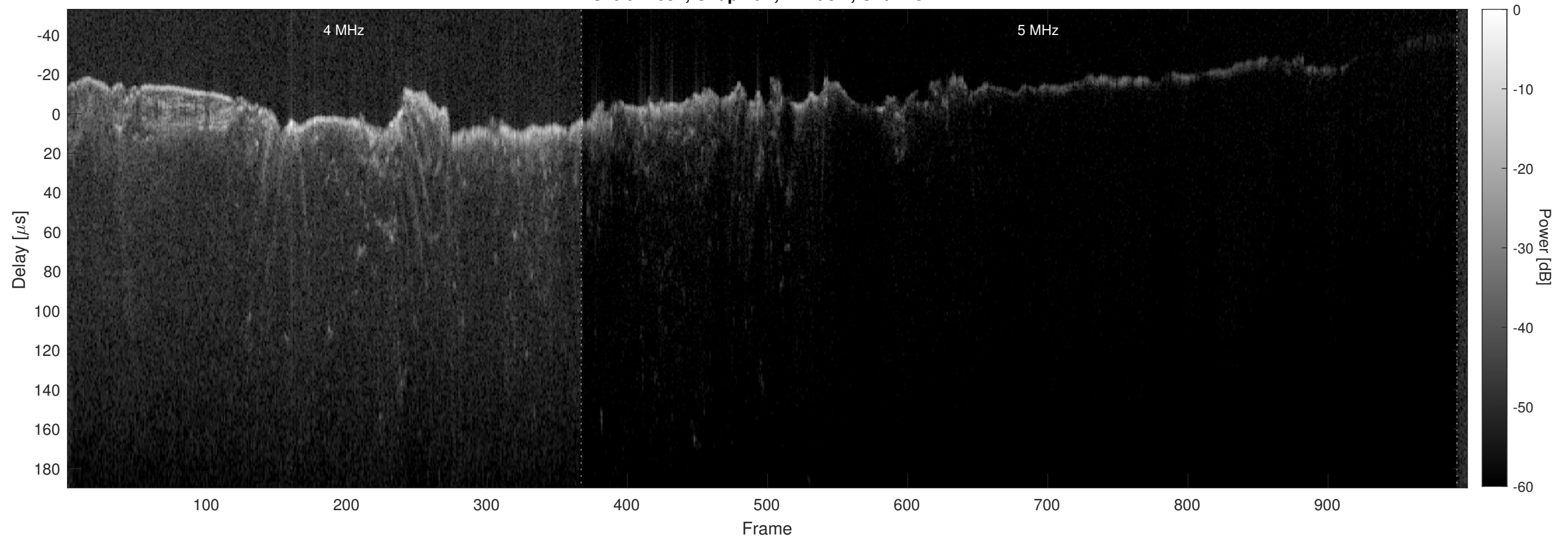
Orbit 12632, Chapman, Window, Channel 2
