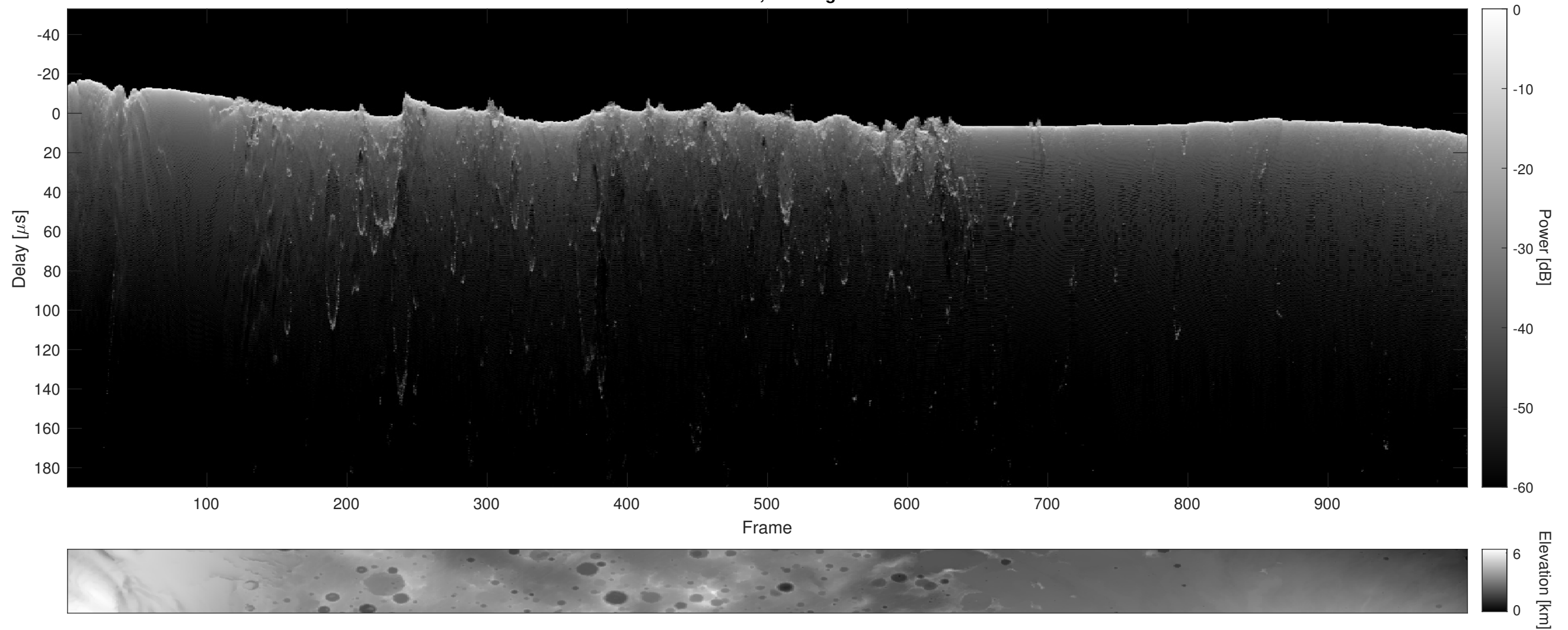
Orbit 12632, Cluttergram
