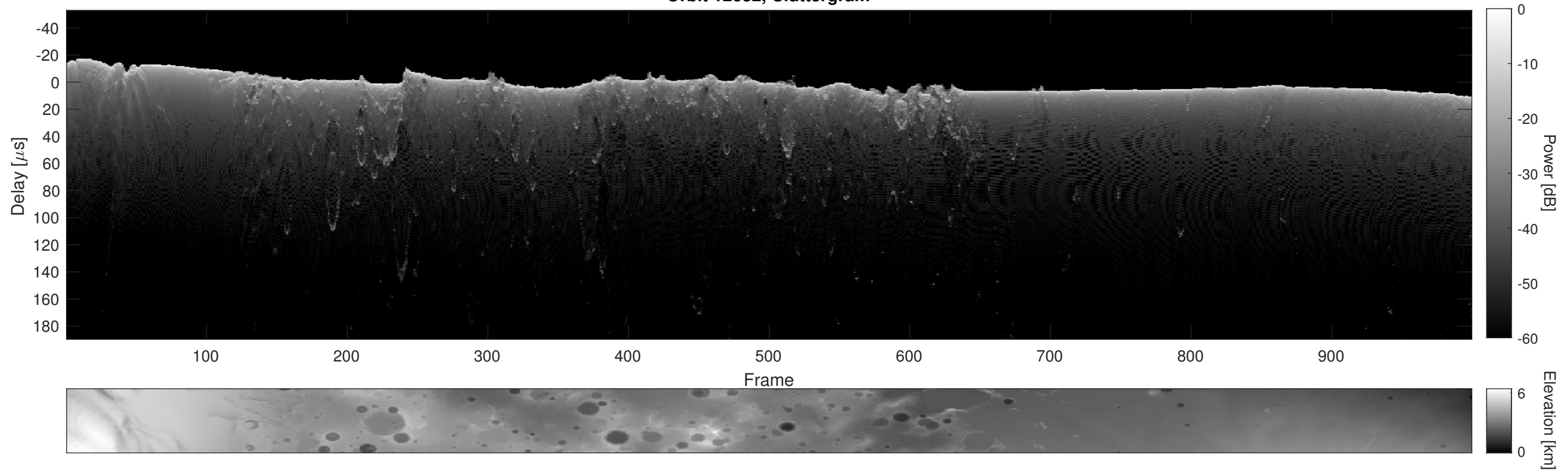
Orbit 12632, Cluttergram
