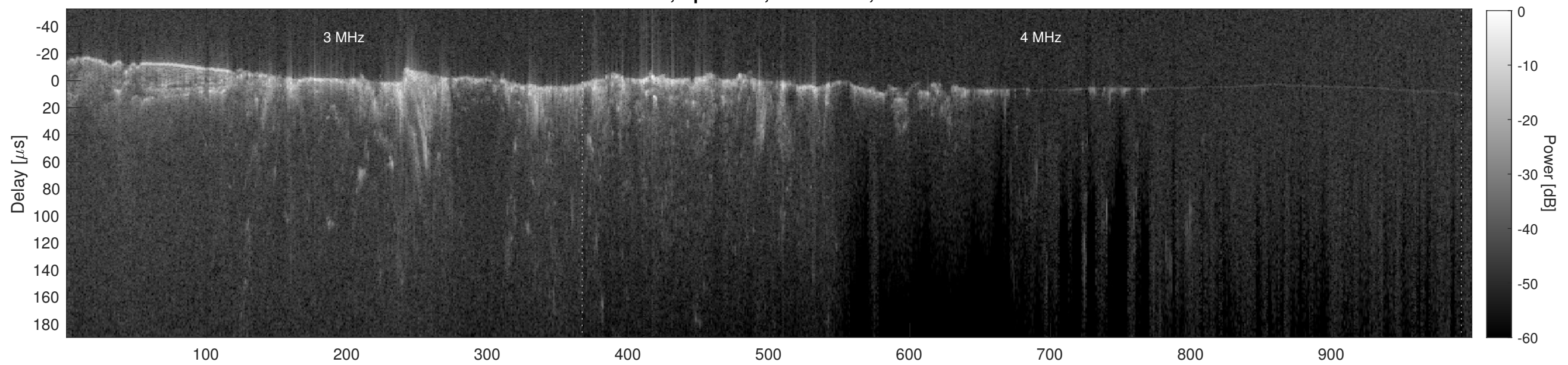
Orbit 12632, Cluttergram
