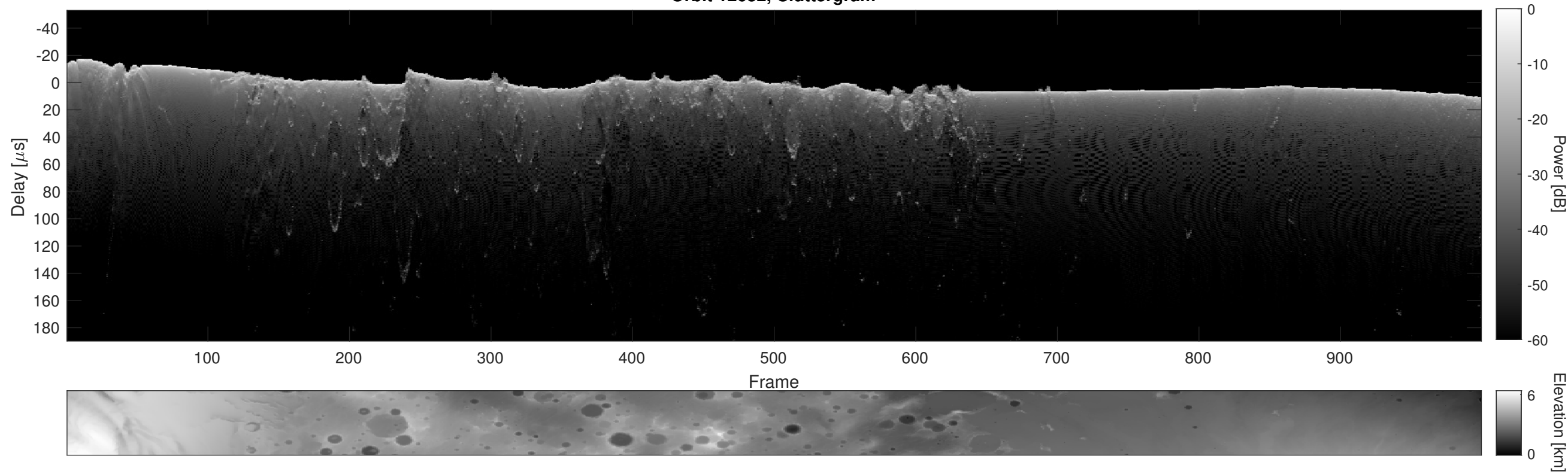
Orbit 12632, Cluttergram
