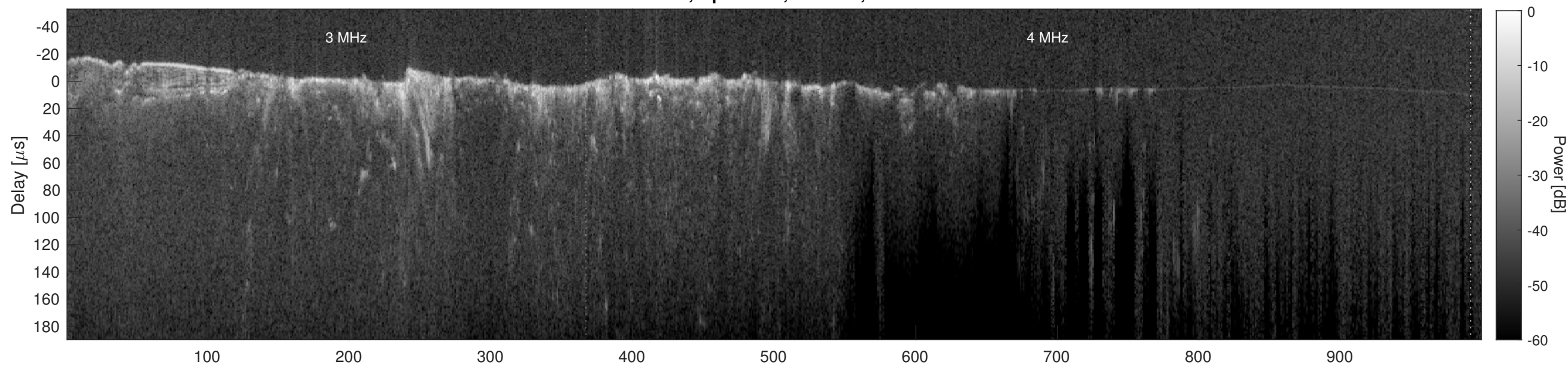
Orbit 12632, Cluttergram
