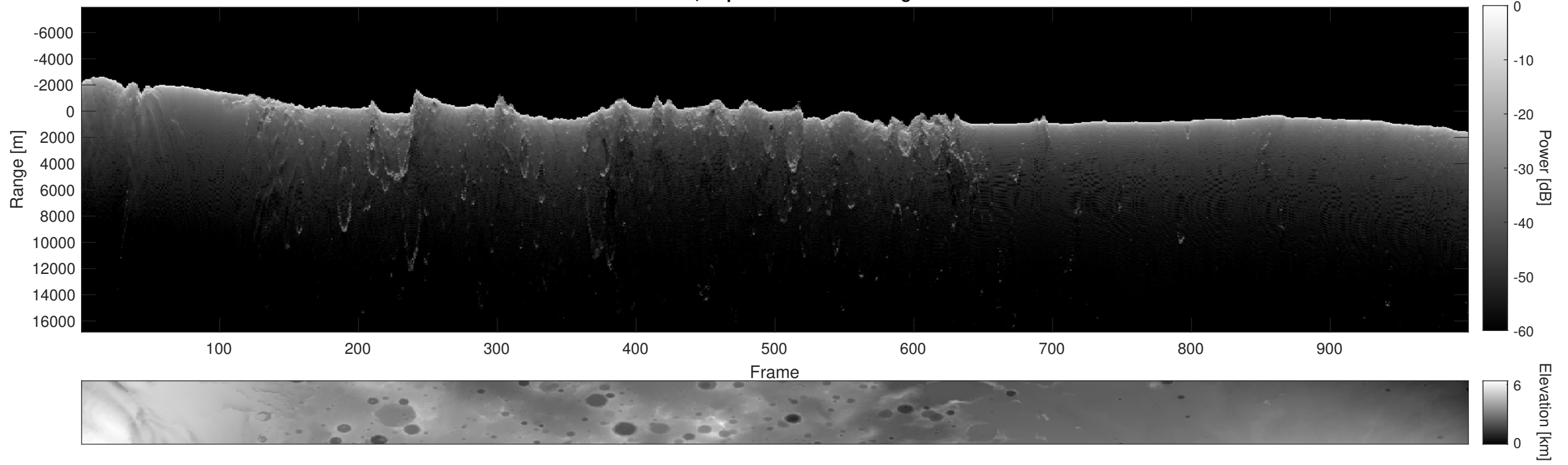
Orbit 12632, Depth-Corrected Cluttergram
