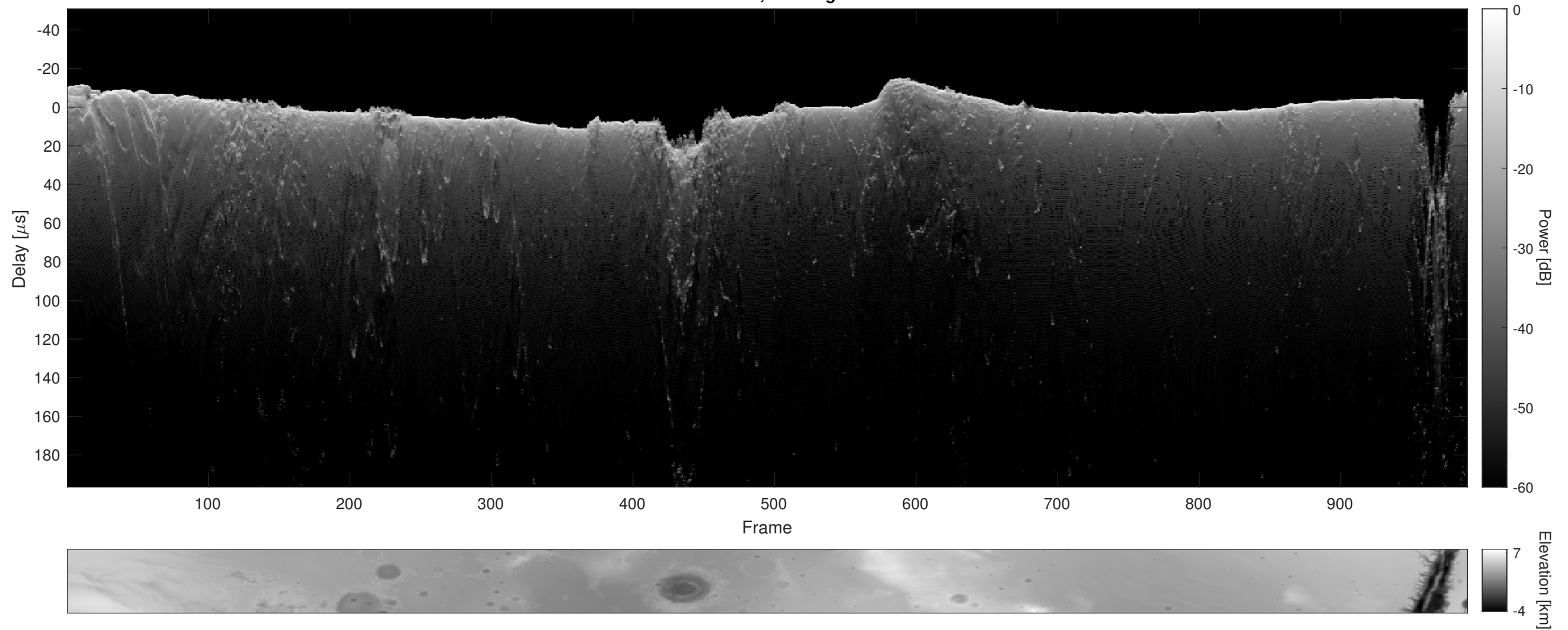
Orbit 12635, Cluttergram
