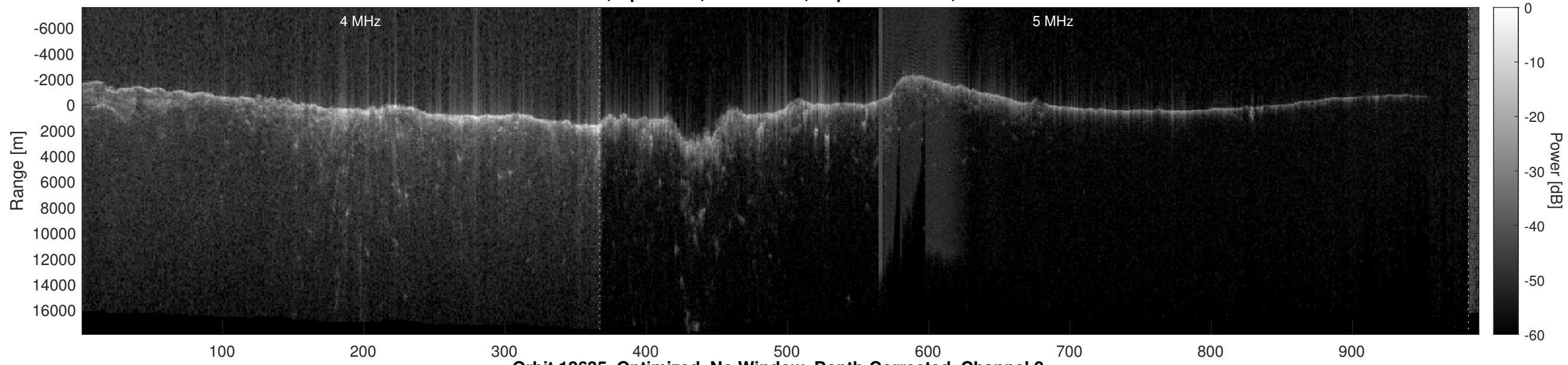
Orbit 12635, Optimized, No Window, Depth-Corrected, Channel 2
