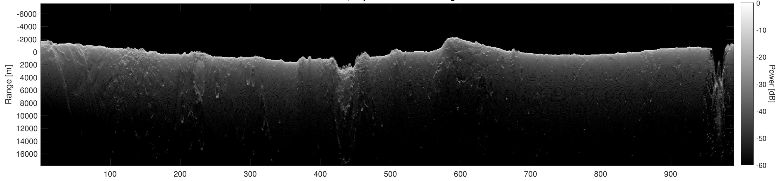
Orbit 12635, Depth-Corrected Cluttergram
