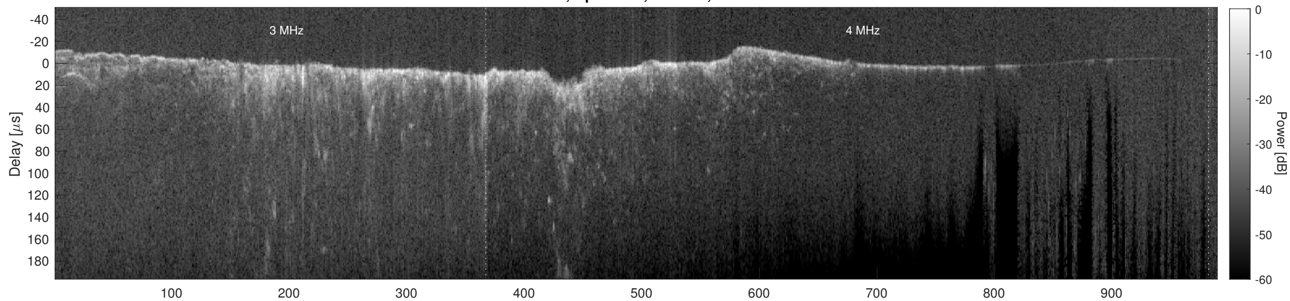
Orbit 12635, Cluttergram
