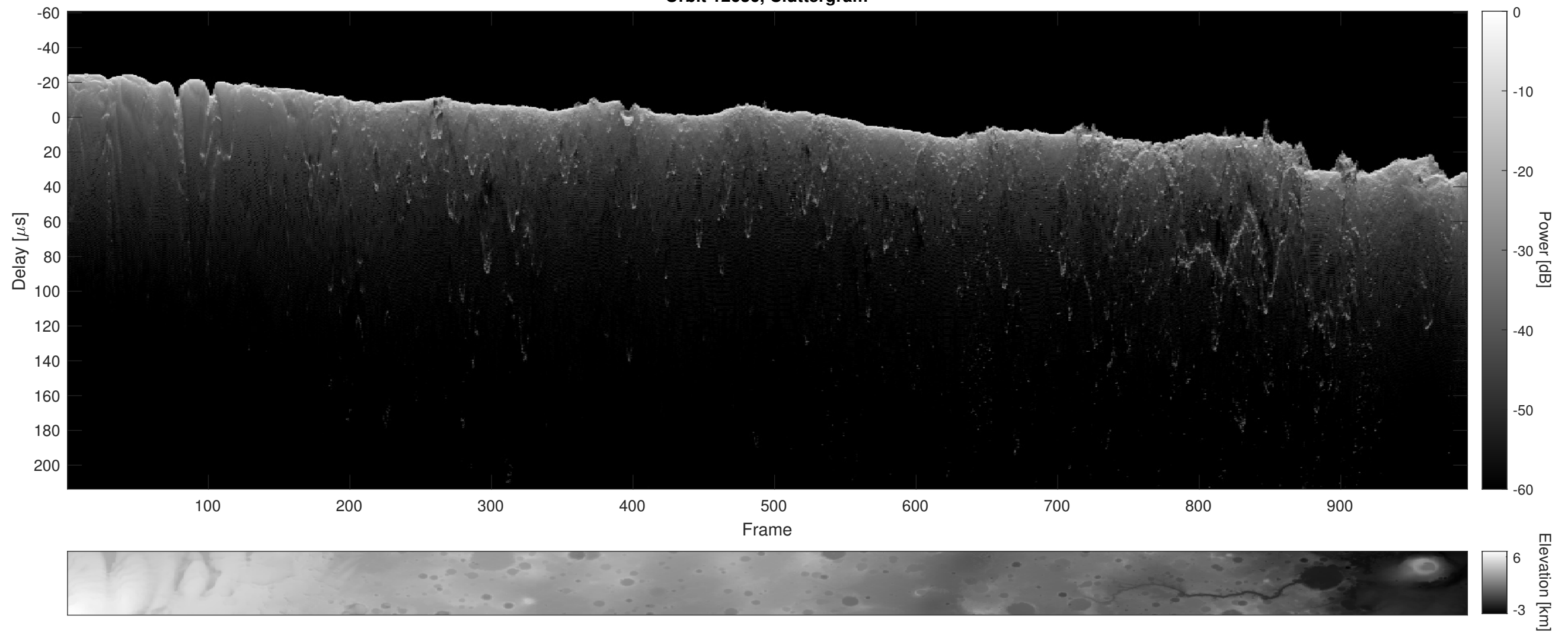
Orbit 12636, Cluttergram
