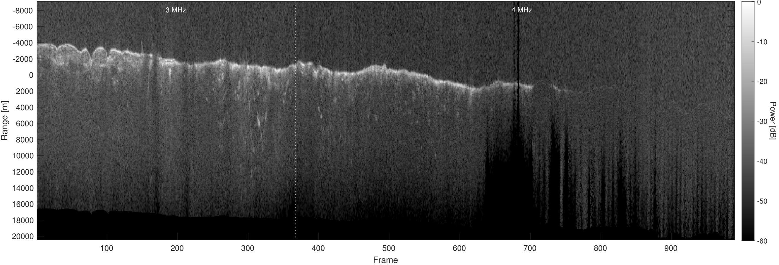
Orbit 12636, Optimized, Window, Depth-Corrected, Channel 2
