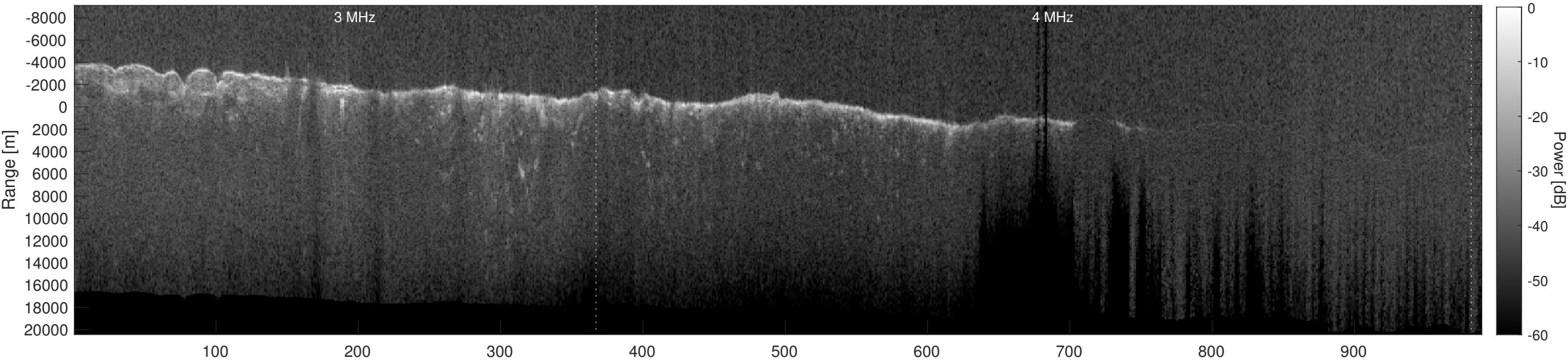
Orbit 12636, Depth-Corrected Cluttergram
