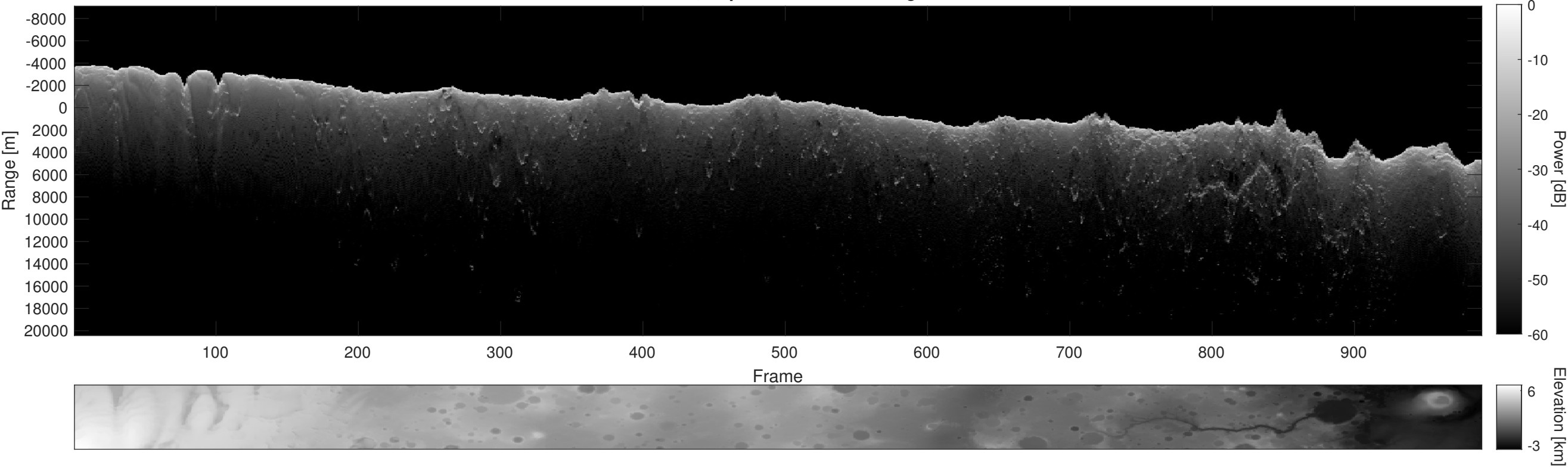
Orbit 12636, Depth-Corrected Cluttergram
