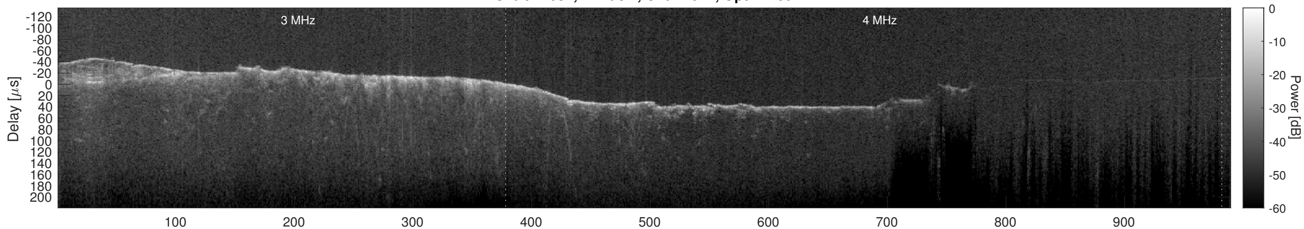
Orbit 12637, Cluttergram
