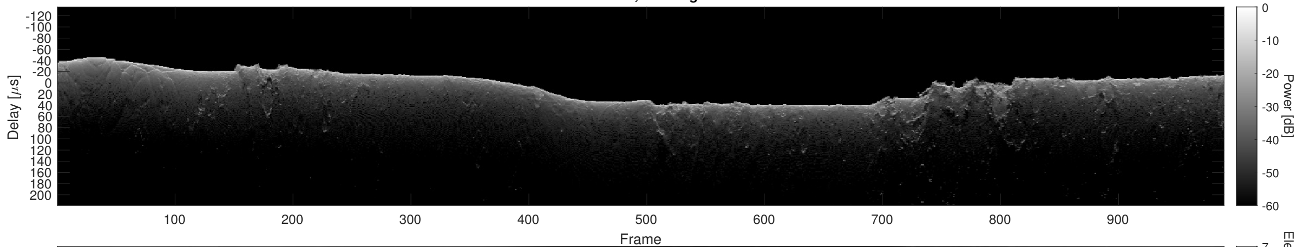
Orbit 12637, Cluttergram
