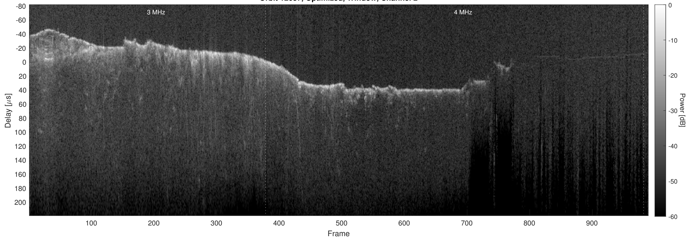
Orbit 12637, Optimized, Window, Channel 2
