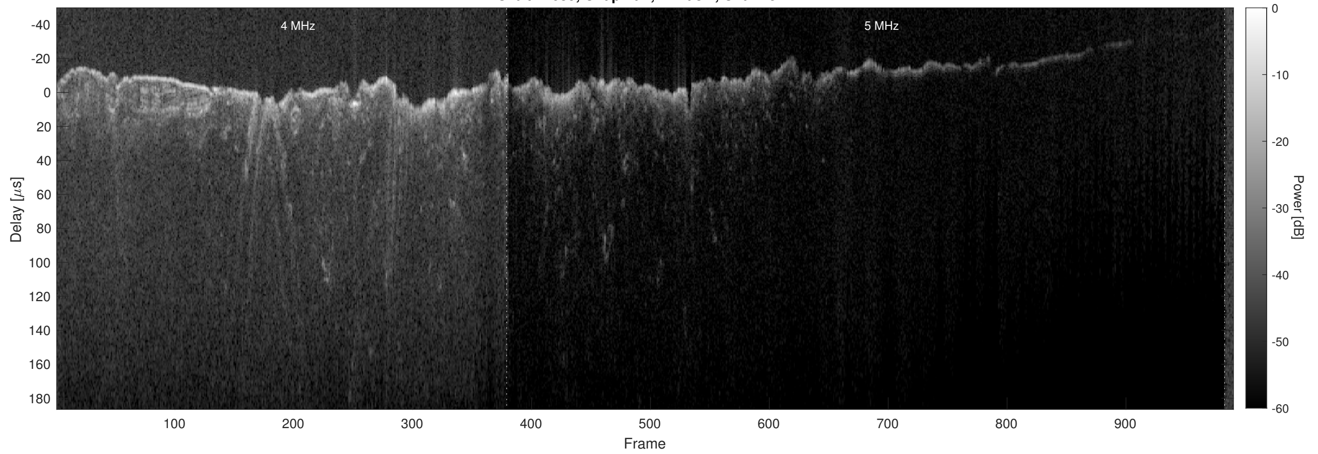
Orbit 12639, Chapman, Window, Channel 2
