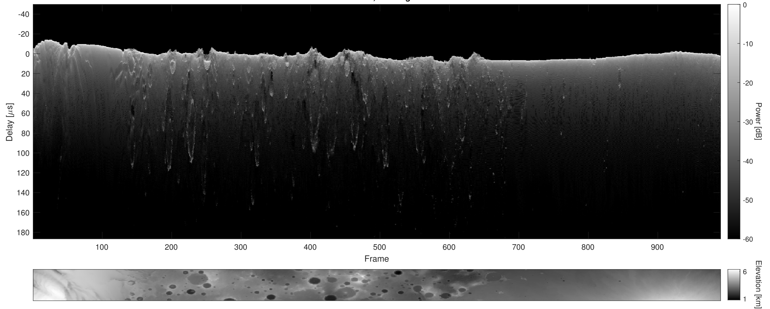
Orbit 12639, Cluttergram
