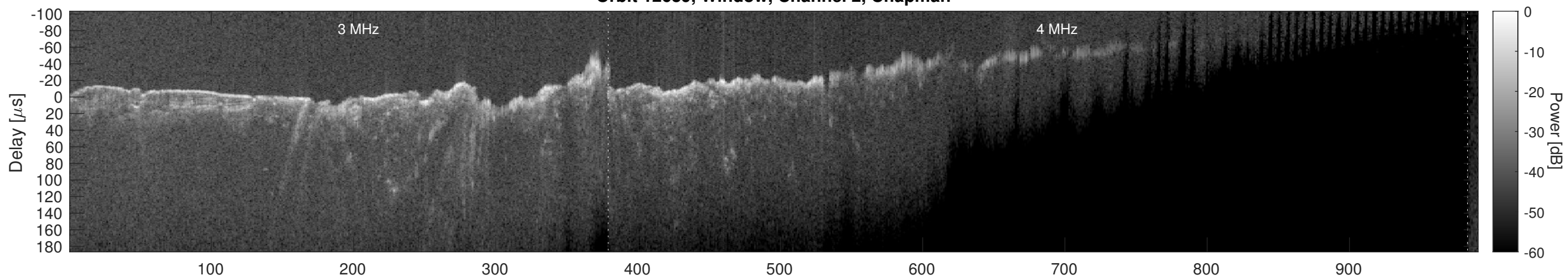
Orbit 12639, Window, Channel 2, Optimized
