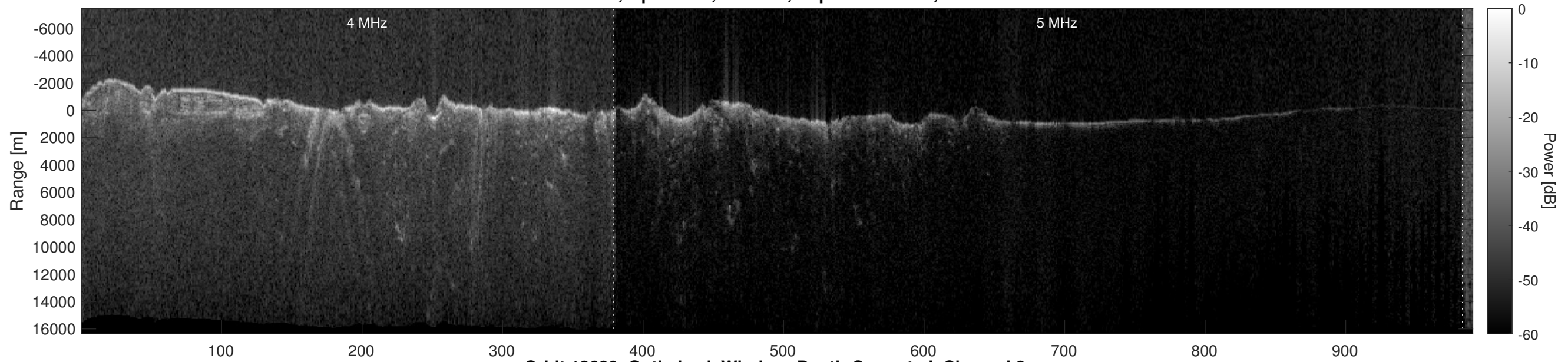
Orbit 12639, Optimized, Window, Depth-Corrected, Channel 2
