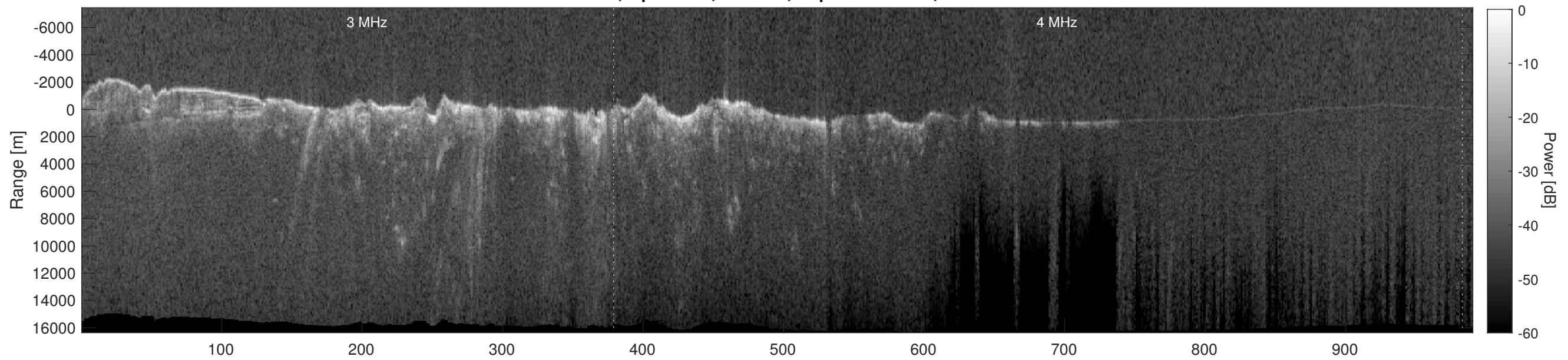
Orbit 12639, Depth-Corrected Cluttergram
