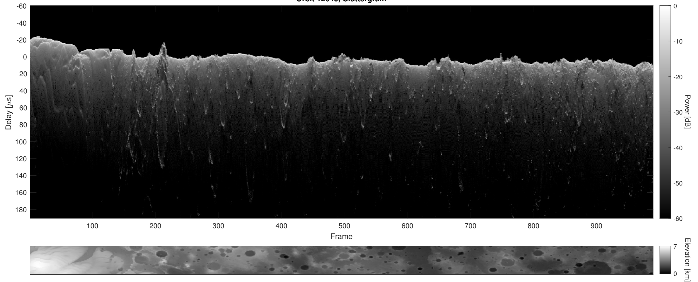
Orbit 12640, Cluttergram
