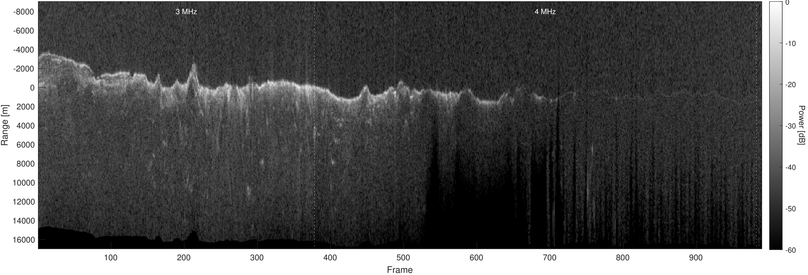
Orbit 12640, Optimized, Window, Depth-Corrected, Channel 2
