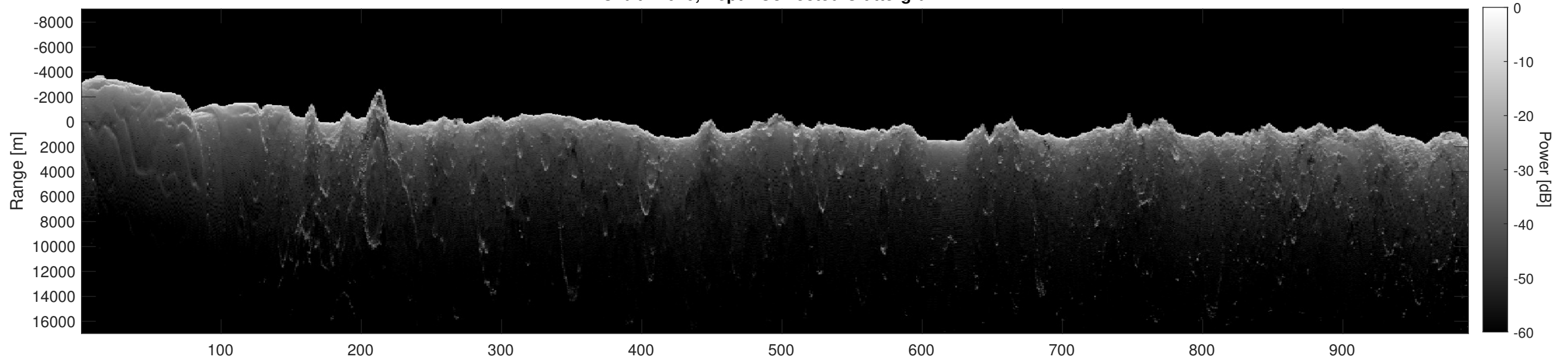
Orbit 12640, Depth-Corrected Cluttergram
