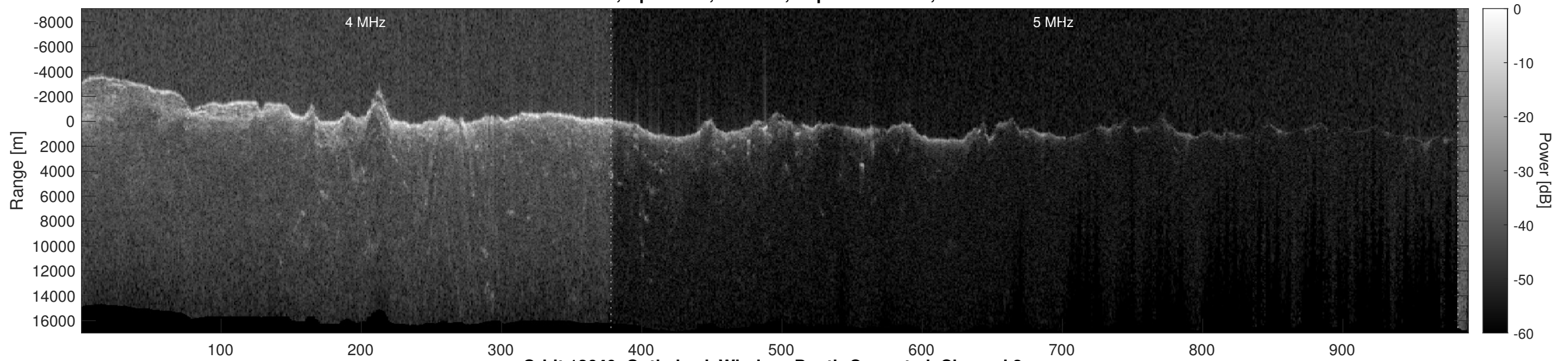
Orbit 12640, Optimized, Window, Depth-Corrected, Channel 2
