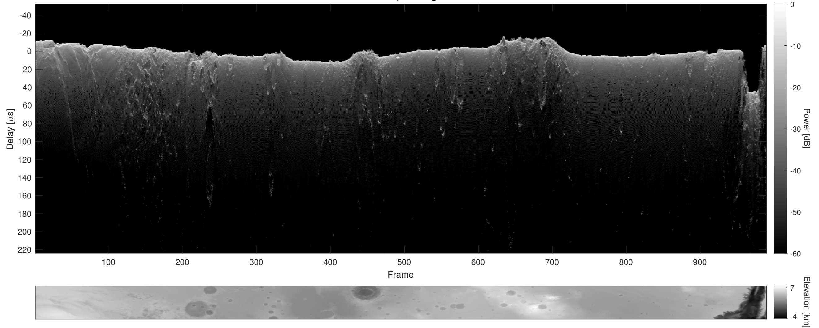
Orbit 12642, Cluttergram
