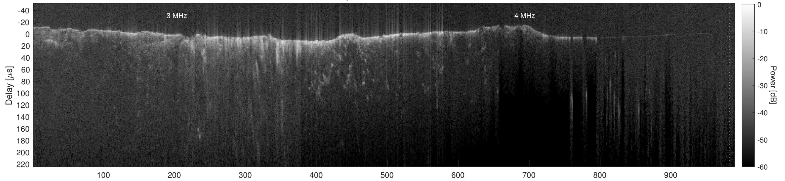
Orbit 12642, Cluttergram
