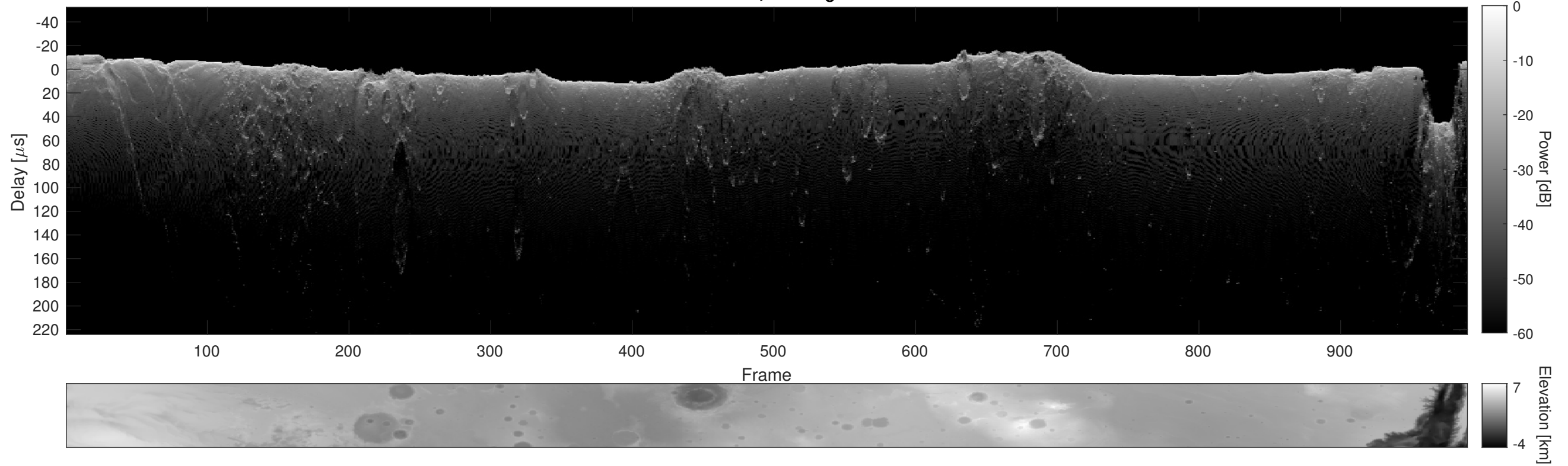
Orbit 12642, Cluttergram
