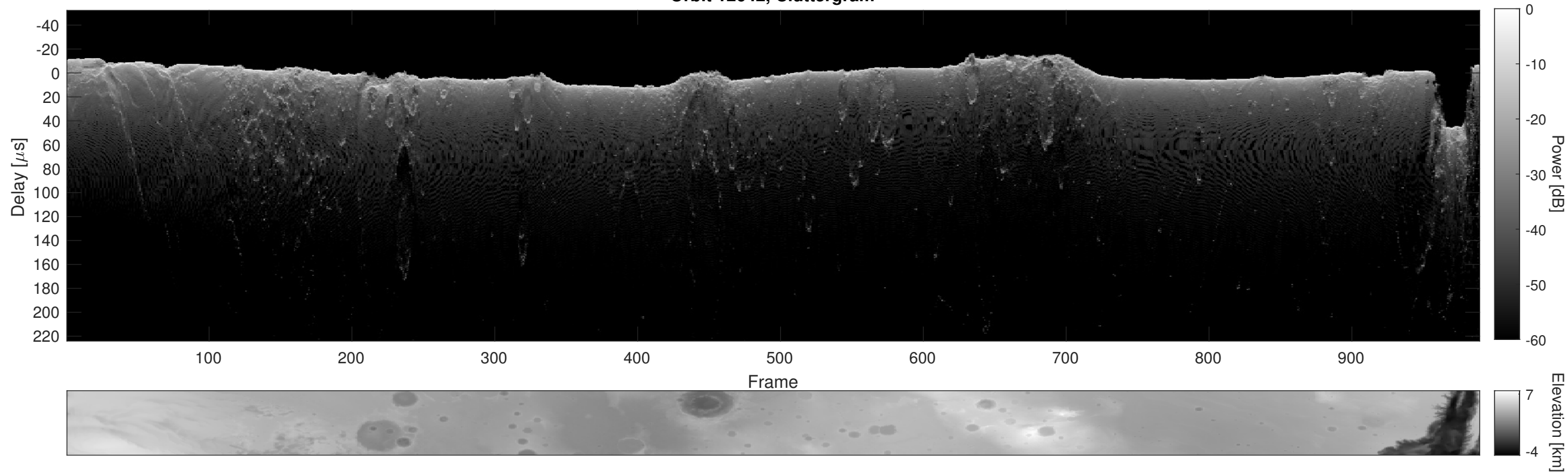
Orbit 12642, Cluttergram
