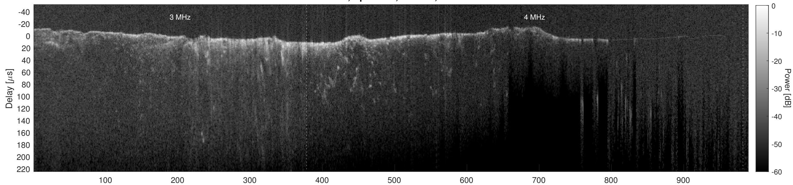
Orbit 12642, Cluttergram
