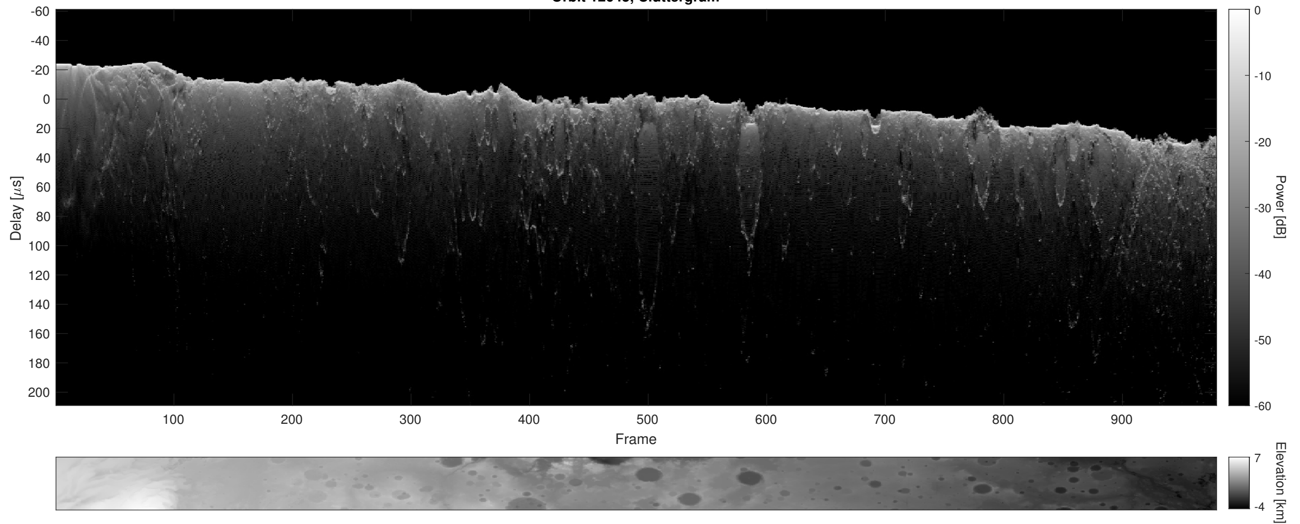
Orbit 12645, Cluttergram
