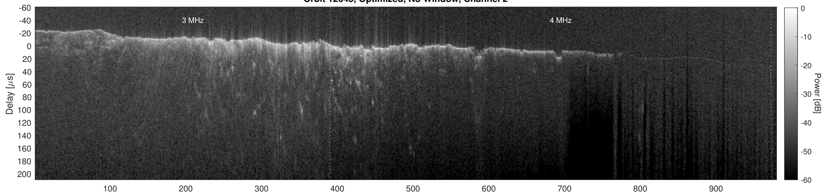
Orbit 12645, Cluttergram
