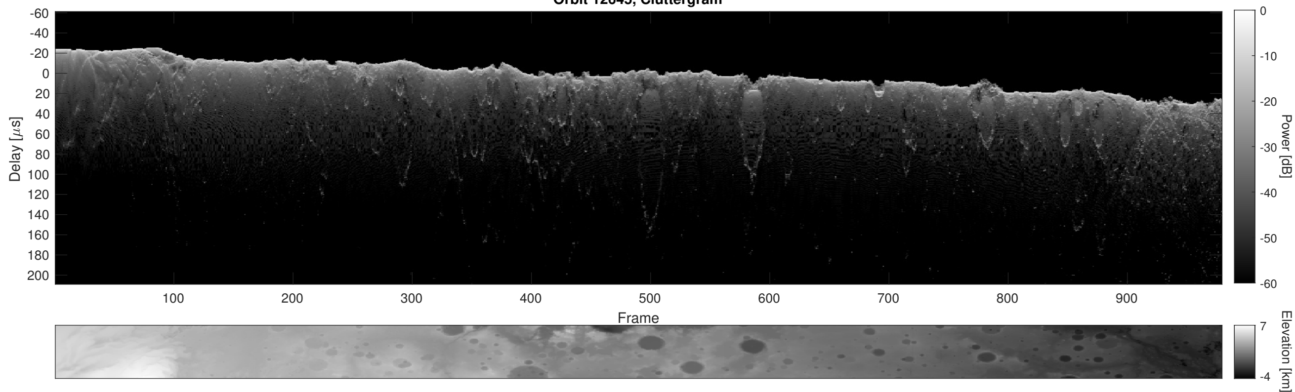
Orbit 12645, Cluttergram
