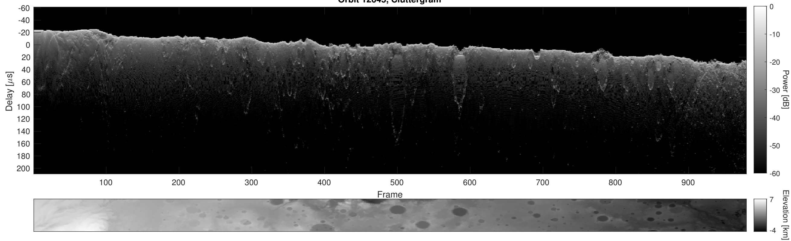
Orbit 12645, Cluttergram
