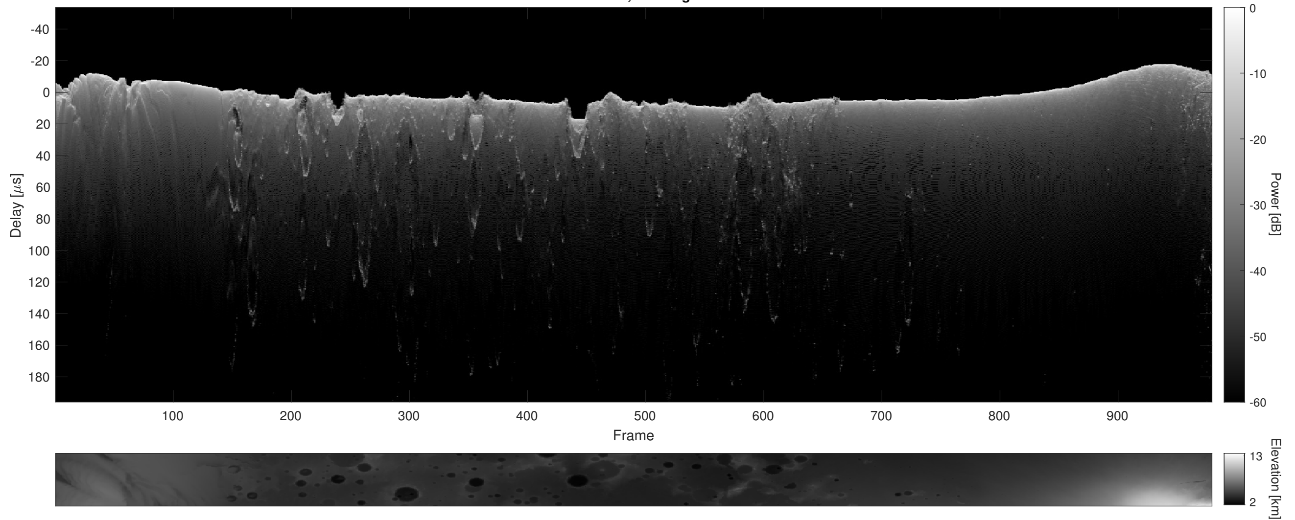
Orbit 12646, Cluttergram
